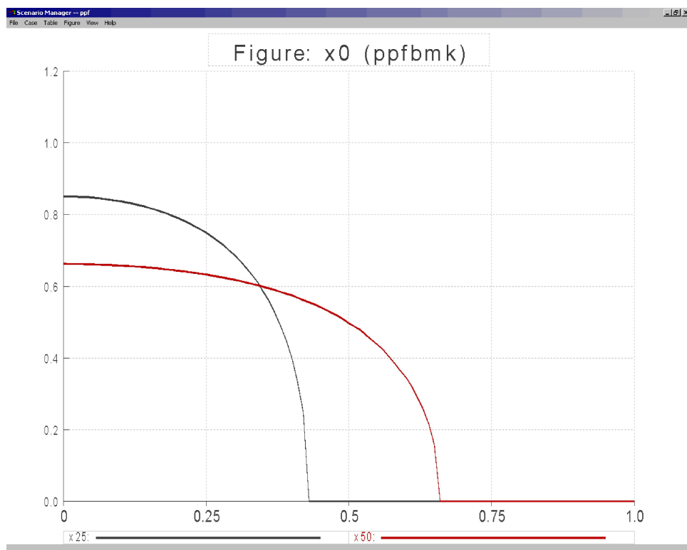
Figure 4: Figure X0 from PPF.SCN
